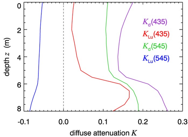
Fig. 6. Selected diffuse attenuation functions.
