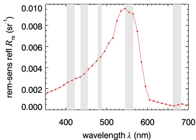
Fig. 7. Remote-sensing reflectance. The red dots show the wavelengths of the HydroLight run; the gray bars show the nominal VIIRS bands.
