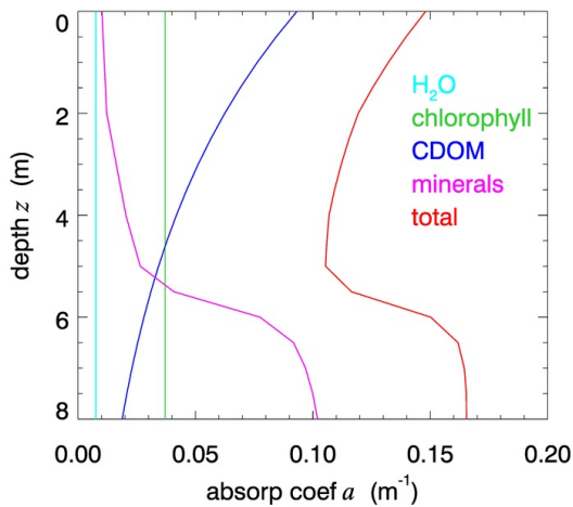
Fig. 1. Component and total absorption coefficients at 445 nm, for the hypothetical water body.
